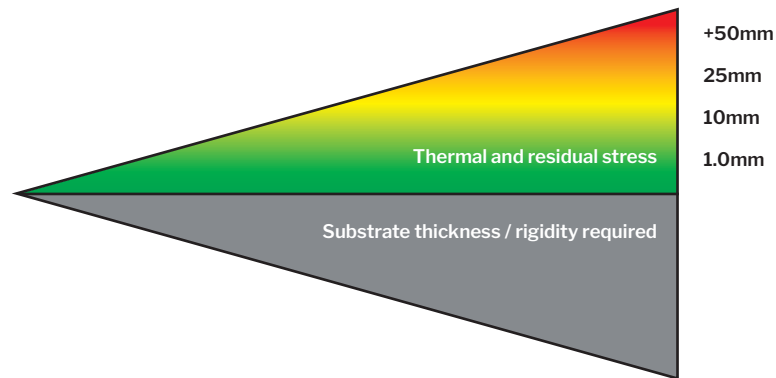
Figure 11: A visual demonstration of the typical increase in scaffold (substrate) thickness/rigidity as more layers are deposited.
