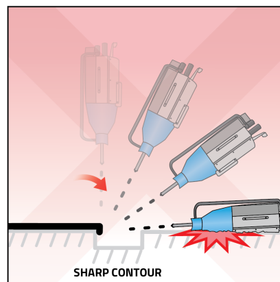
Figure 7 [Left]: Demonstration that an obstruction above the surface of deposition does not allow for the nozzle to reach the location of intended deposition
