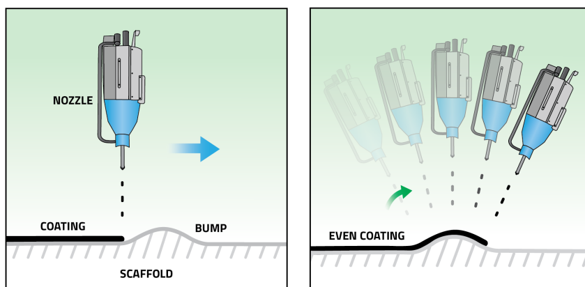
Figure 3: As the nozzle scans across the surface (image on left), a uniform coating is applied.
