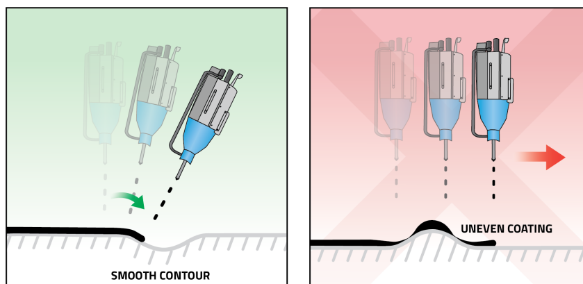
Figure 4 [Left]: Once again, as the surface angle changes, the nozzle angle rotates to follow the contour of the bump while maintaining scanning speed and offset distance, resulting in an even, uniform coating.
