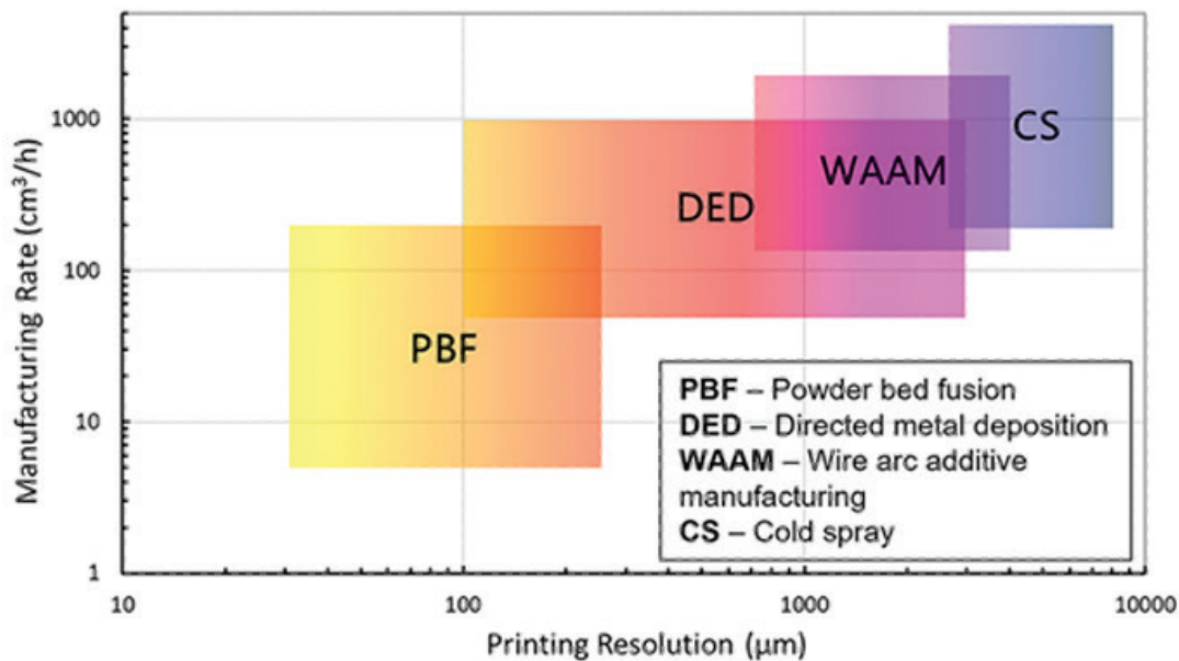
Figure 2: Comparison of the deposition (manufacturing) rates and feature resolutions of CSAM, SLM, EBM, DED, and WAAM for AM of structural materials.
