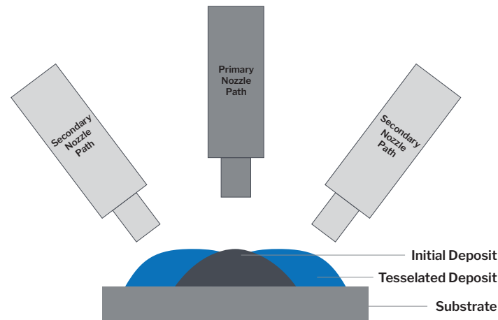
Figure 13: Depiction of a simple tessellation angle approach, in which a primary line is deposited and then two subsequent lines are deposited on the slope of the primary line to offset the peaking effect caused by cold spray physics
