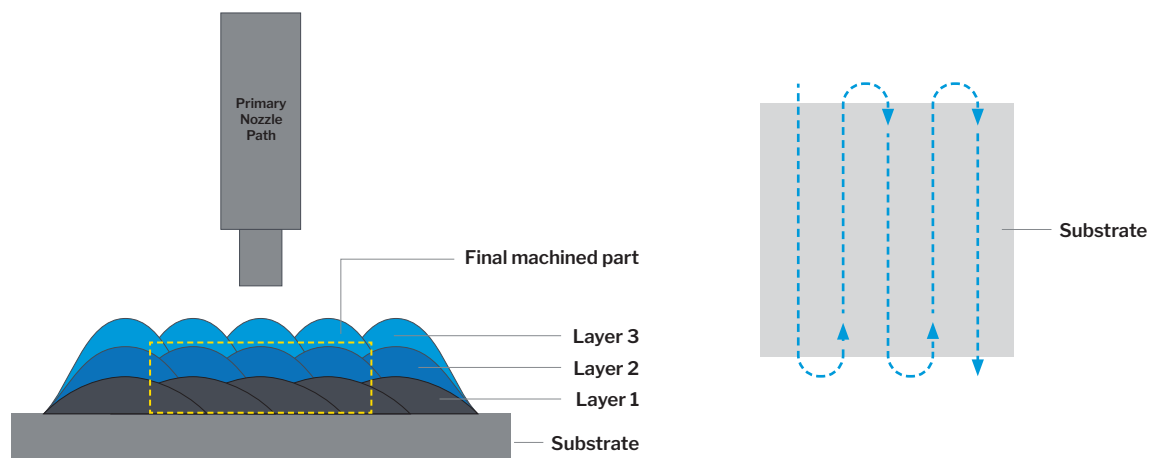
Figure 14: [Left] Layers that are multiple lines wide are created with the nozzle maintaining normal angle to the substrate [Right] a birds-eye view of the path plan shows how these adjacent lines are created for each individual layer
