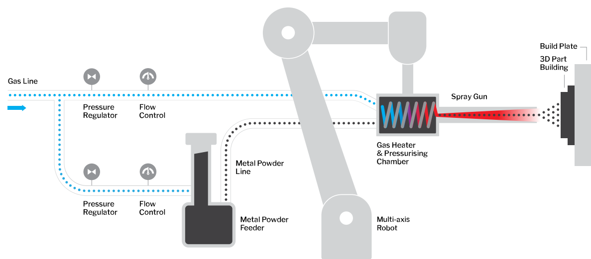
Figure 1: CSAM technology process resulting in deposition
