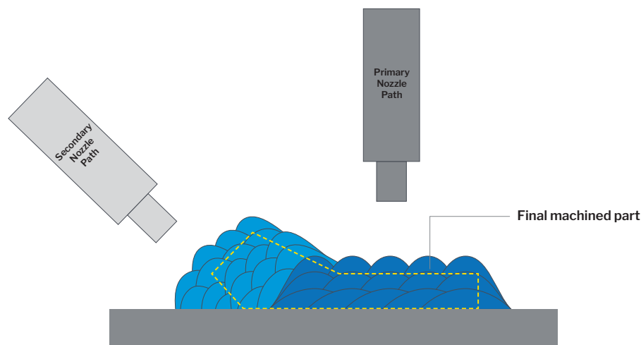
Figure 15: A demonstration of how step-over overlaps and off-angle strategies can be leveraged to build near-net shaped final parts using cold spray
