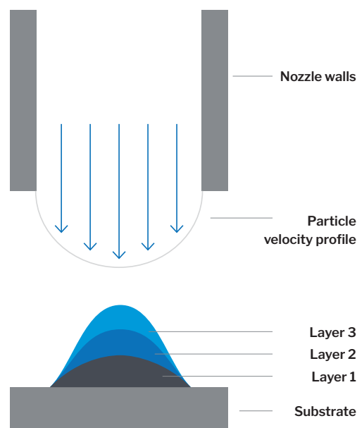
Figure 12: A nozzle cross section is shown with the gas/powder mixture's particle velocity profile, causing the increasingly observable mounding effect of each single-line layer
