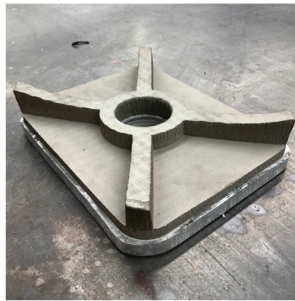
Figure 17: As sprayed and machine-finished
