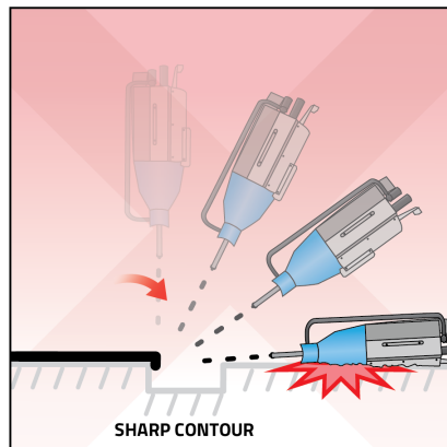
Figure 6: A sharp 90-degree edge presents a challenge to maintain a normal angle to the surface and thus a low likelihood of successful deposition at/near the edge.
