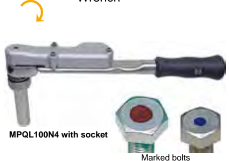
Marked bolts
