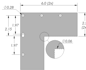
Polycarbonate corner stop.
