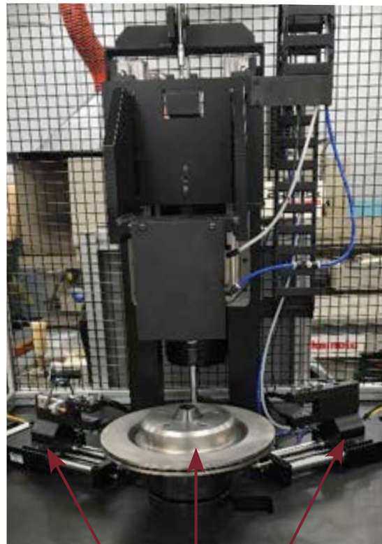
Rotating Fixture
